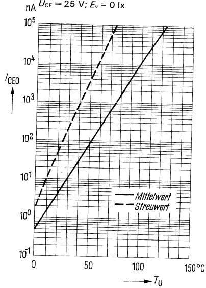
Reststrom I_{CE0} = f(T_U) U_{CE} = 25 \text{ V}; E_v = 0 \text{ V}
