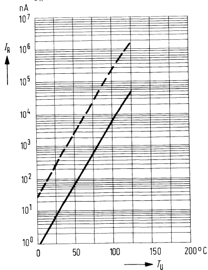
Dunkelstrom I_R = f(T_U) U_R = 10 V
