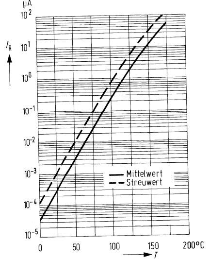
Dunkelstrom I_R = f(T) E = 0 ; U_R = 1\text{ V}
