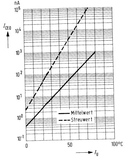
Reststrom I_{CEO} = f(T_U) U_{CE} = 30 \text{ V}; E_V = 0 \text{ lx}
