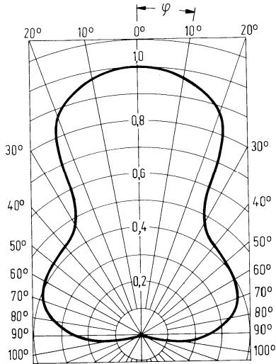
Richtcharakteristik I_{rel} = f(\varphi)
