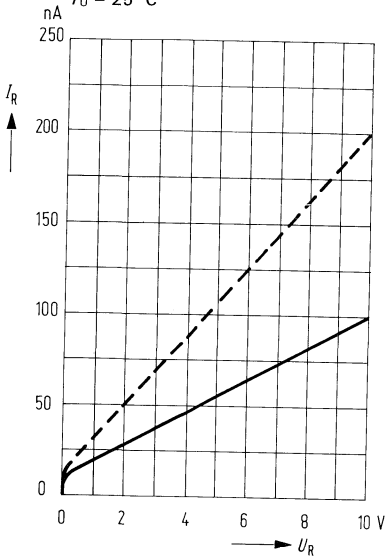
Dunkelstrom I_R = f(U_R) T_U = 25^\circ\text{C}
