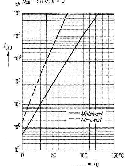
Reststrom I_{CE0} = f(T_U)
