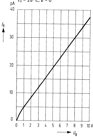
Dunkelstrom I_R = f(U_R) T_U = 25^\circ\text{C}; E = 0
