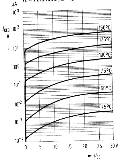
Dunkelstrom I_{CEO} = f(U_{CE}) T_U = \text{Parameter}; E = 0
