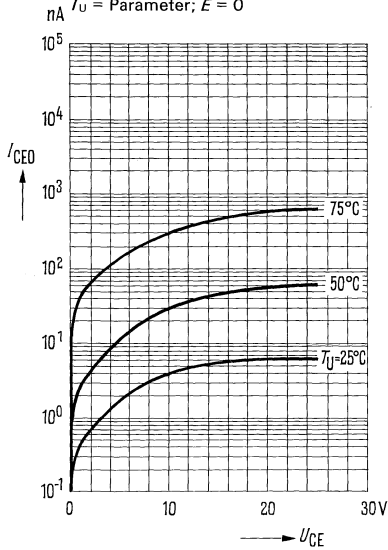
Reststrom I_{CE0} = f(U_{CE})
