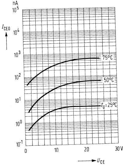
Reststrom I_{CEO} = f(U_{CE}) T_U = \text{Parameter}; E_V = 0 \text{ lx}
