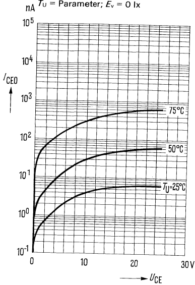
Reststrom I_{CE0} = f(U_{CE}) T_U = \text{Parameter}; E_v = 0 \text{ V}
